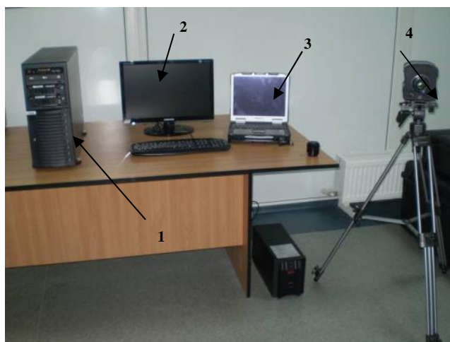
Fig.2 – Thermal signature analyzing system
